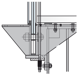
Connection at Base
