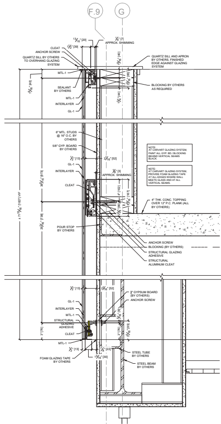
2 VERTICAL SECTION DETAIL SCALE: 3" = 1'-0"
