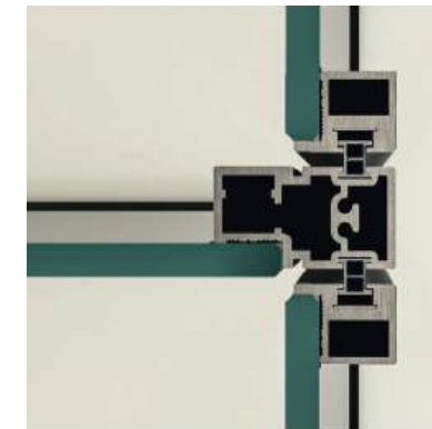
Partition module- Detail of low hinges, right door and left door
