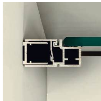
Fixed module - Side upright section.
