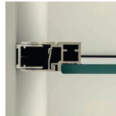
Partition module - Upright section on wall side with shower area
