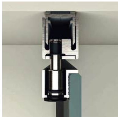
Hinged door - Detail of the profile and upper hinge
