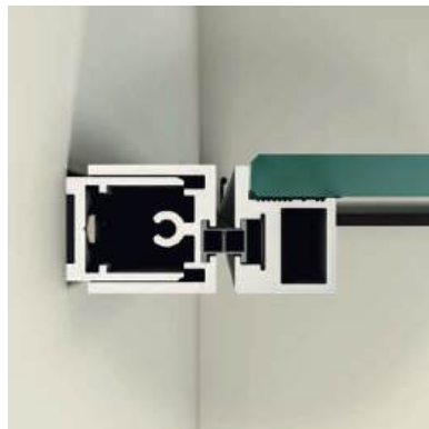
Hinged door - Detail of the magnetic seal and side profile
