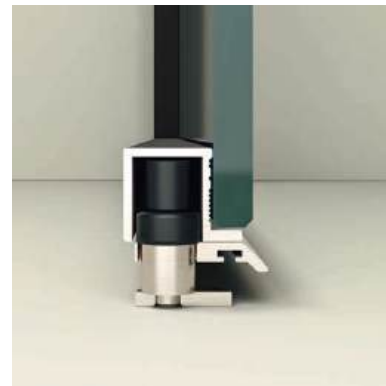
Hinged door - Section of the lower profile and hinge of the DRY door
