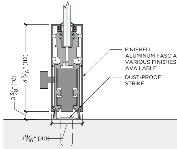
TYPICAL DETAILS
