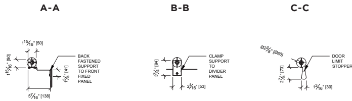
VERTICAL SECTIONS
