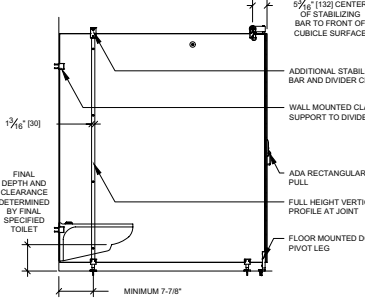
A-A VERTICAL SECTION
