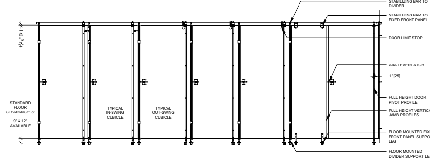
INTERIOR ELEVATION
