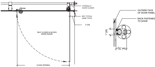
PLAN VIEWS
