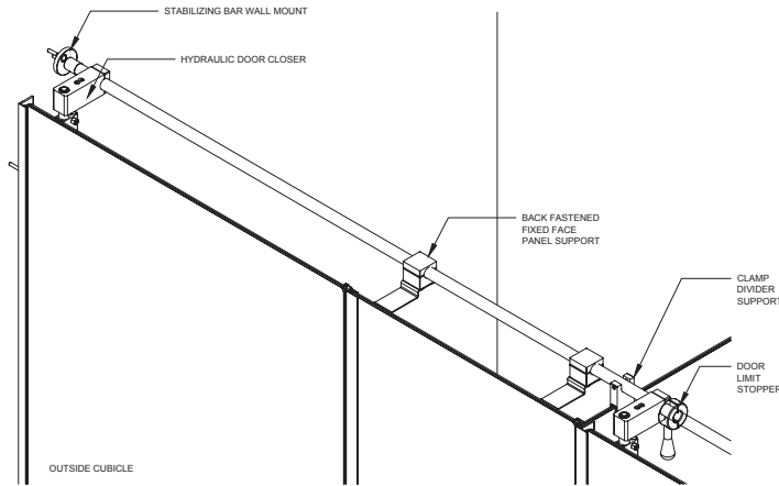
EXTERIOR ISOMETRIC
