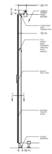
VERTICAL SECTION
