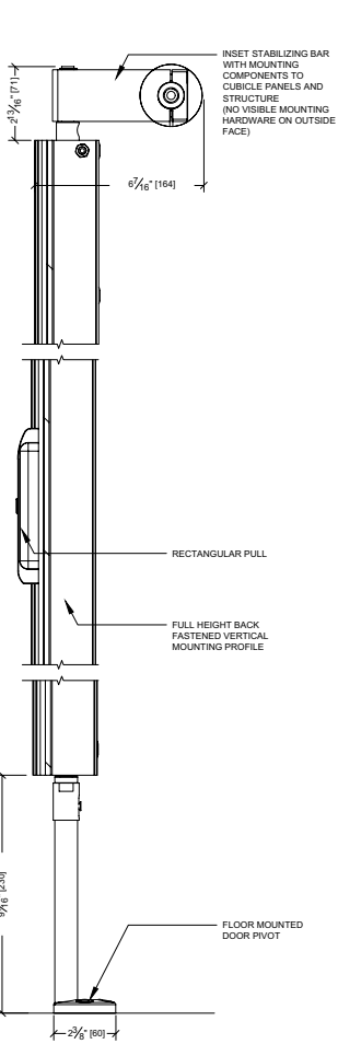
VERTICAL SECTION
