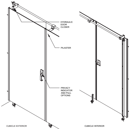
TYPICAL ISOMETRICS
