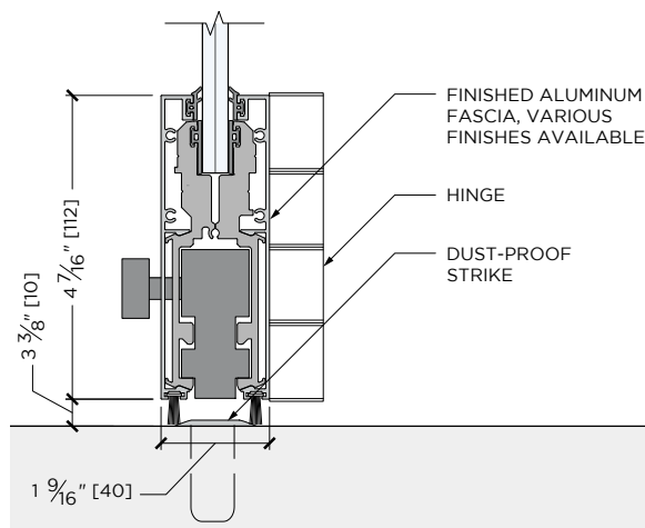
TYPICAL DETAILS
