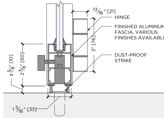
VERTICAL SECTION @ BASE SHOE
